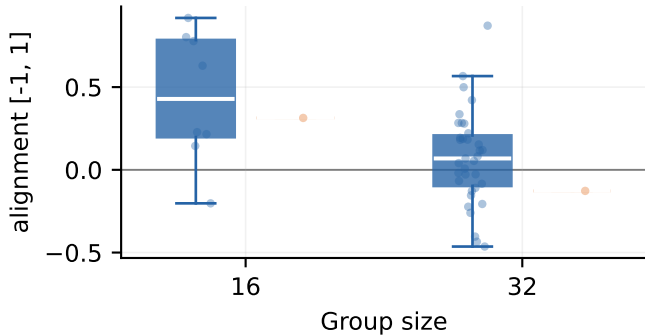
Pursuit alignment
