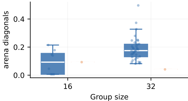
Predator distance
